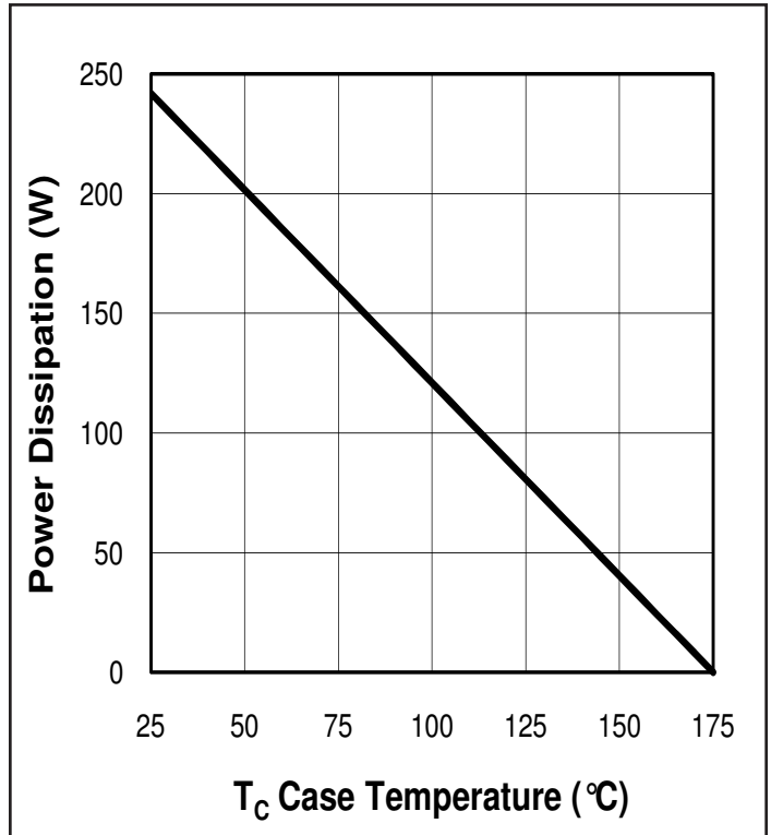
Figure 6. Power Derating
