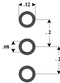
TO-247-3
